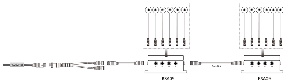
BSA09 radar control box connection diagram
