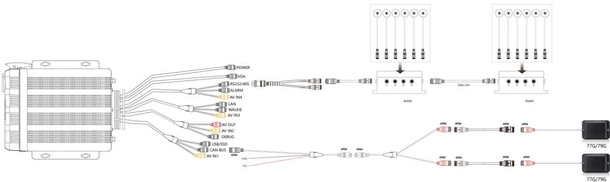
Schematic of DVR connecting two types of radar
